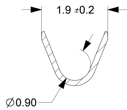
SECTION Y-Y SCALE 20:1 ROTATED 180°
