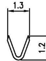
B-B SECTION
