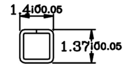
Section C-C
