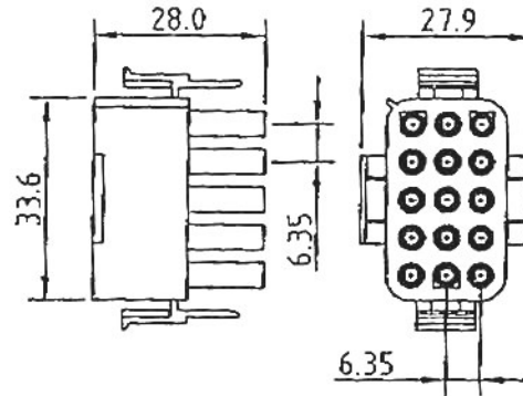
H6350-15PSW0000
