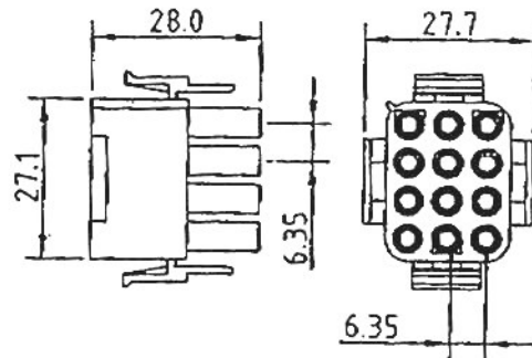
H6350-12PSW0000
